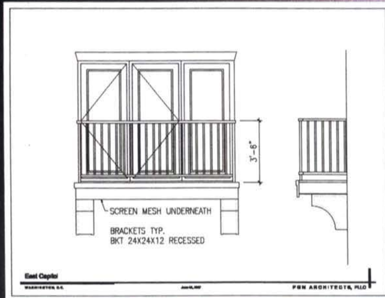
Balcony Detail
